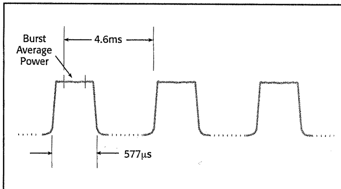
Figure 3. GSM RF pulse train. The Model 2800 has the speed to capture consecutive 577µs pulses.
