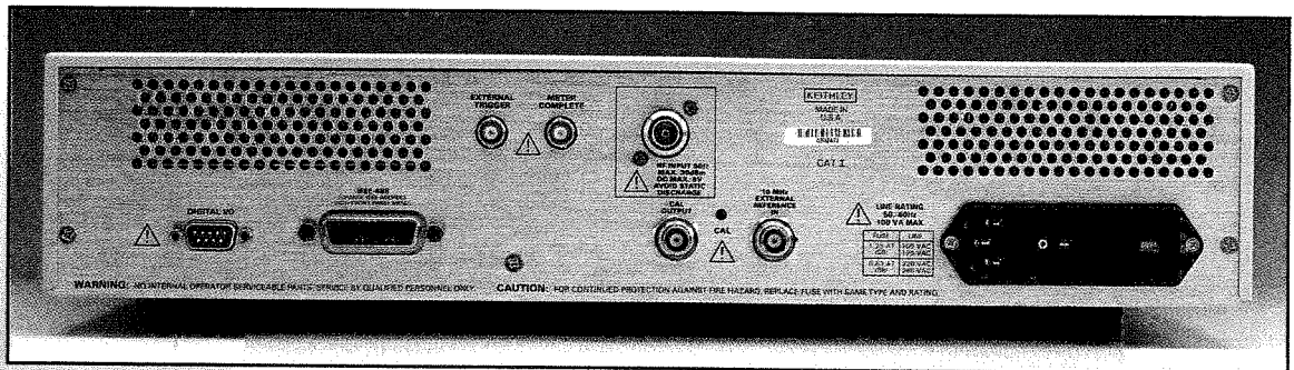
Figure 8. Rear panel of 2800 showing Type N input connector, external reference input, calibration output, external trigger and measurement complete BNC connectors, IEEE-488 connector, and DB9 digital I/O relay control lines connector.
