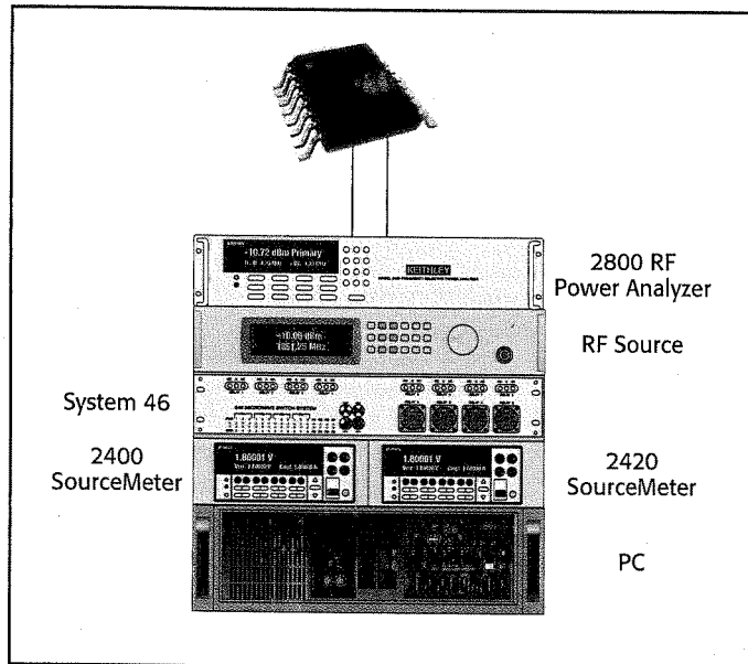
Figure 6. RFIC power amplifier functional test system. Throughput is greatly enhanced with instrumentation optimized for production test.
